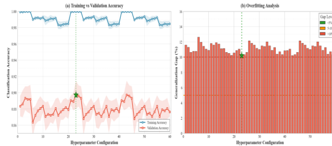
Fig. 4. Comparison of hyperparameter configuration and overfitting gap
