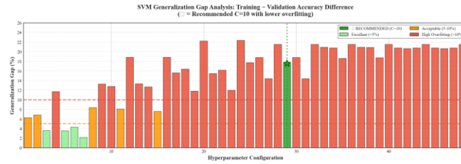
Fig. 1. Comparison of SVM training and validation testing
