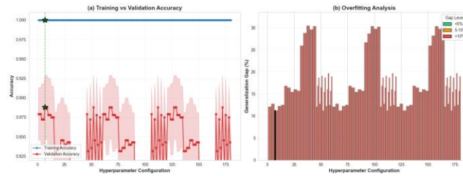
Fig. 3. Hyperparameter training and validation results graph and overfitting
